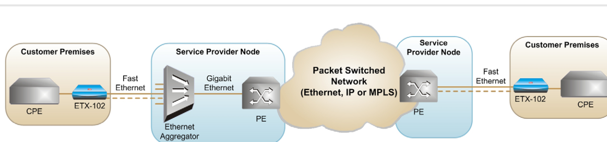
Figure 1. Providing Managed Ethernet Services over a PSN using ETX-102
