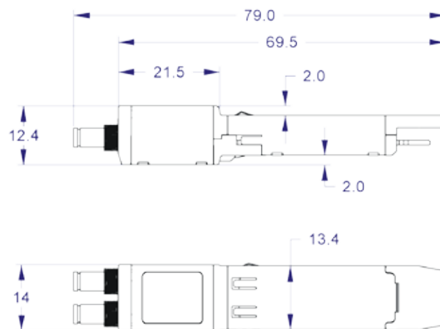
Figure 2 Physical Dimensions
